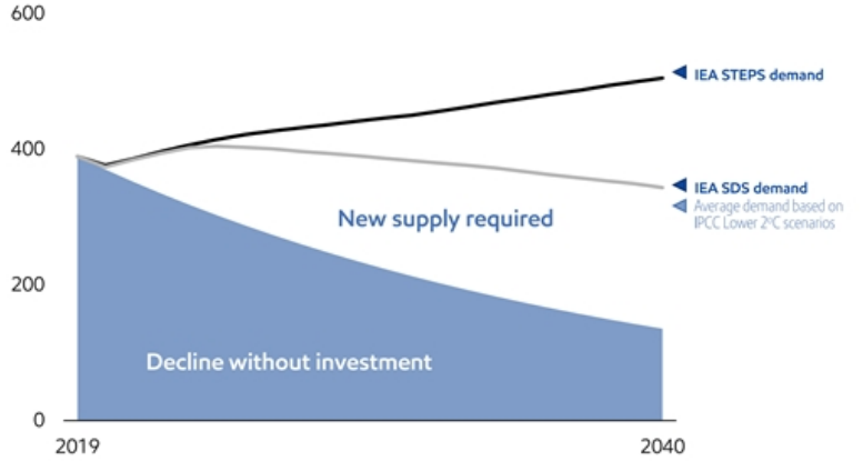
GLOBAL NATURAL GAS SUPPLY ESTIMATES Billion cubic feet per day
