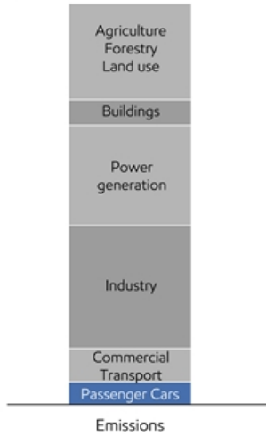
2010 GLOBAL EMISSIONS BY SOURCE 49 GT/yr CO 2 e
