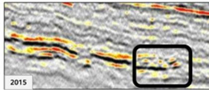
EVOLUTION OF SEISMIC DATA IN GUYANA
