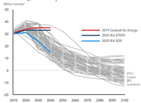
Global energy-related CO 2 emissions 113
