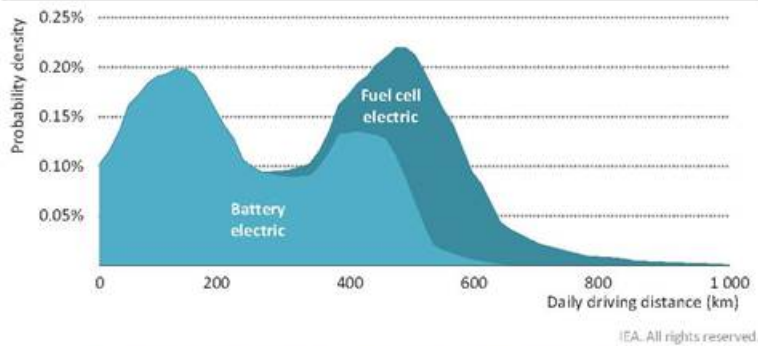
Figure 3.24 ▶ Heavy trucks distribution by daily driving distance, 2050
