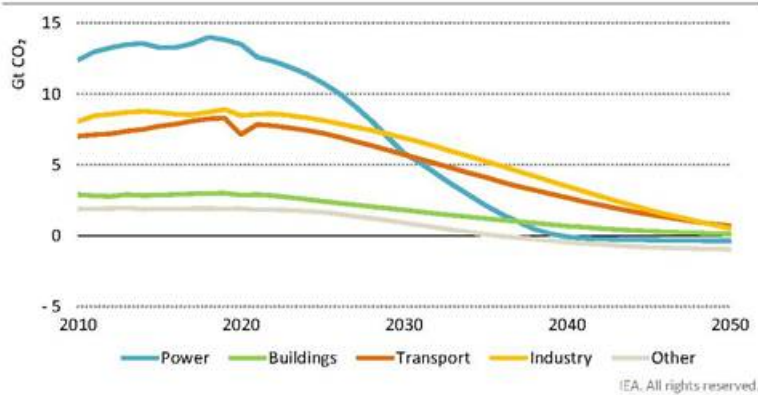
Figure 3.1 ▶ CO 2 emissions by sector in the NZE
