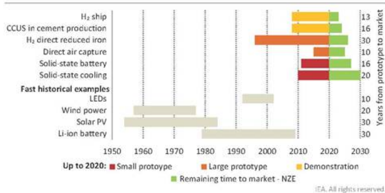
Figure 4.23 ▶ Time from first prototype to market introduction for selected technologies in the NZE and historical examples
