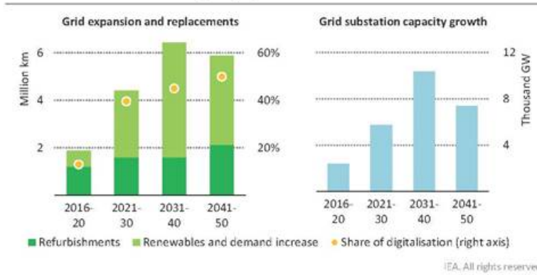
Figure 4.19 ▶ Annual average electricity grid expansion, replacement and substation capacity growth in the NZE
