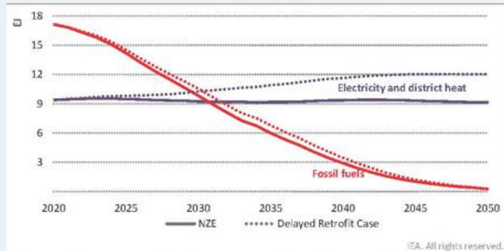
Figure 3.31 ▶ Global residential space heating and cooling energy demand in the NZE and Delayed Retrofit Case
