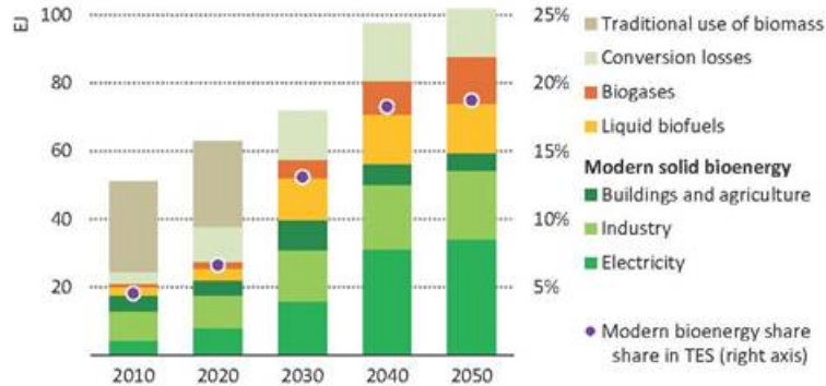
Figure 2.20 ▶ Total bioenergy supply in the NZE
